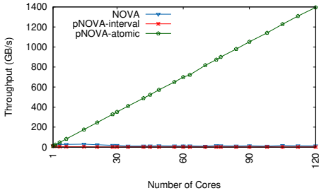
Figure 5: DRBM workload results in FxMark
